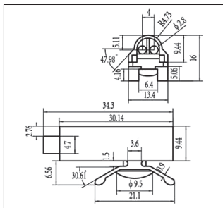
∅8 mm. NFT-A-33
